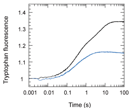
FIGURE 6: Enhancement on tryptophan fluorescence on binding 60\ \mu\text{M} AMPPNP to 2\ \mu\text{M} S1dC: wt (blue trace); S236A mutant (black trace). Conditions were as in Figure 5. Fitting a biexponential to the data between 0.1 and 10\ \text{s} yielded rate constants of 3.4\ \text{s}^{-1} (amplitude = 0.17 ) and 0.24\ \text{s}^{-1} (amplitude = 0.14 ) for the S236A construct. For the wild-type construct values were 5.4\ \text{s}^{-1} (amplitude = 0.085 ) and 0.92\ \text{s}^{-1} (amplitude = 0.081 ). The fluorescence signal was normalized to 1 for the apo state, so that the total fluorescence enhancement in these records was 31\% for the S236A construct and 16.6\% for the wild type.
