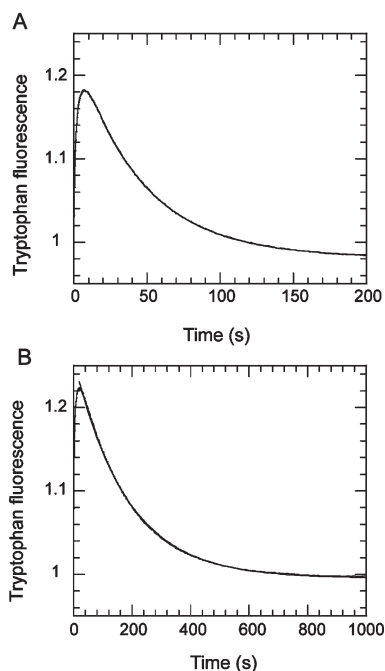
FIGURE 5: Single turnover of 1\ \mu\text{M} ATP by 2\ \mu\text{M} S1dC as monitored by tryptophan fluorescence: (A) wild-type; (B) S236A mutant. The reaction was measured in 40\ \text{mM} NaCl, 10\ \text{mM} Hepes, and 2\ \text{mM} \text{MgCl}_2 at pH 7.5 and 20^\circ\text{C} . The signals were normalized such that the fluorescence of the apo state was equal to 1. Superposed fits to a single exponential yield rate constants of 0.02 and 0.0058\ \text{s}^{-1} , respectively.
