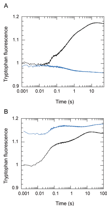
FIGURE 7: (A) Stopped-flow records showing the change in tryptophan fluorescence on binding 50\ \mu\text{M} \text{PP}_i to 2\ \mu\text{M} S1dC (wild-type showing quench in fluorescence (blue trace) and S236A (black trace) showing an enhancement). (B) The fluorescence enhancement on binding 500\ \mu\text{M} \text{PP}_i to 2\ \mu\text{M} S236A at 20^\circ\text{C} (black) or 5^\circ\text{C} (blue). The records are normalized to the fluorescence of the apo state at 20^\circ\text{C} .
